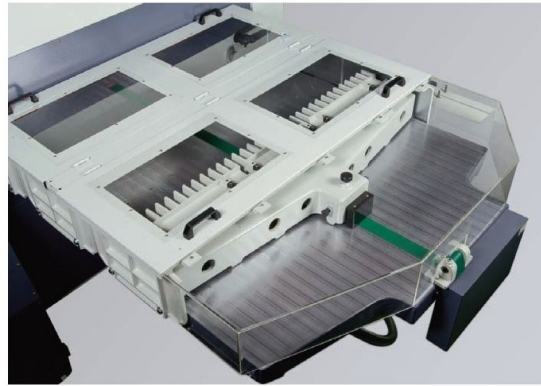
Openable back side cover with safety switch for all model cutting machines
