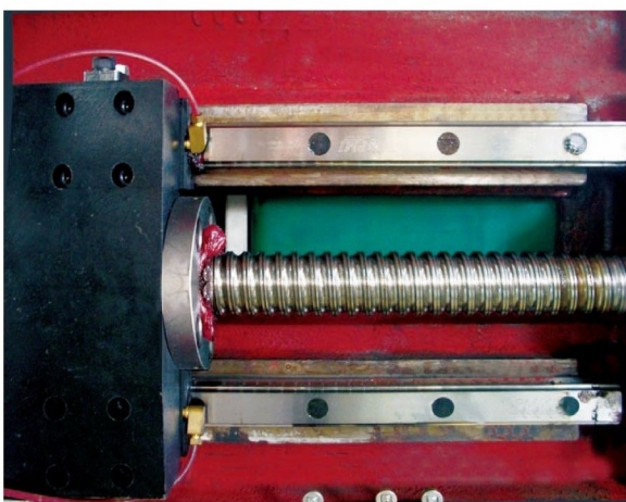
Dual linear rail standard on size 1550 up
